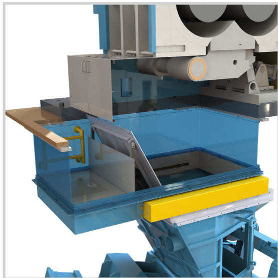
mBox ® with retracted platform (production position)
